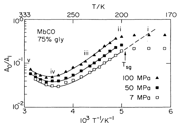
FIG. 2. Plot of r_0 = A_0/A_1 vs 10^3/T for three pressures. Roman numerals signify the five temperature regions defined in the text. The transition temperature T_{sg} is indicated. The dashed line shows the extrapolation from region (iii) for 7 MPa.
