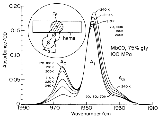
FIG. 1. Absorption spectra of the CO stretch bands of MbCO at 100 MPa. Solvent: 75% glycerol and water mixture, buffered with 100 mM potassium phosphate to pH 6.8. Inset: Cross section through the heme showing the angle \alpha , between the CO dipole and the heme normal.
