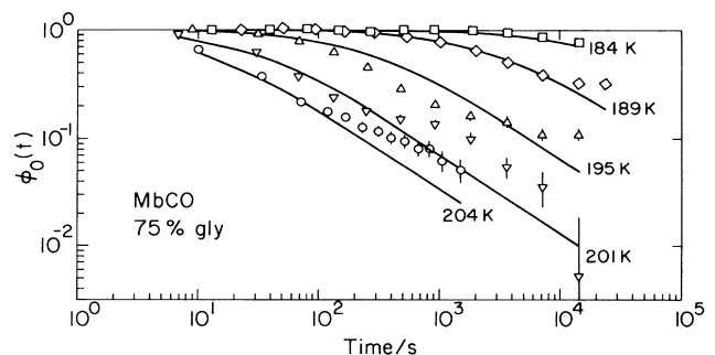
FIG. 4. Relaxation function \Phi_0(t) for the area A_0 vs time. Solid lines are fits with Eqs. (1) and (3) with parameters as given in the text.
