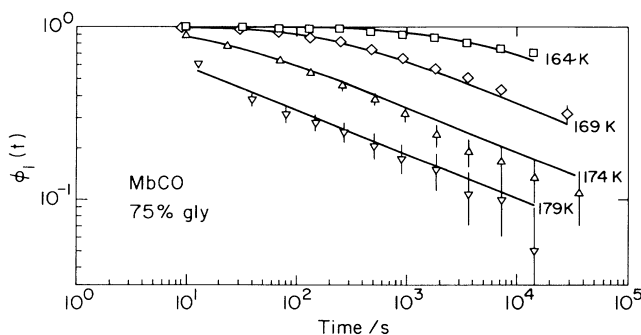
FIG. 3. Relaxation function \Phi_1(t) for the center frequency \nu_0 of the A_0 band vs time. Solid lines are fits with Eqs. (1) and (3) with parameters as given in the text.
